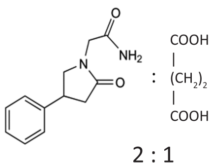
Figure 1 – Structural formula of succinard
