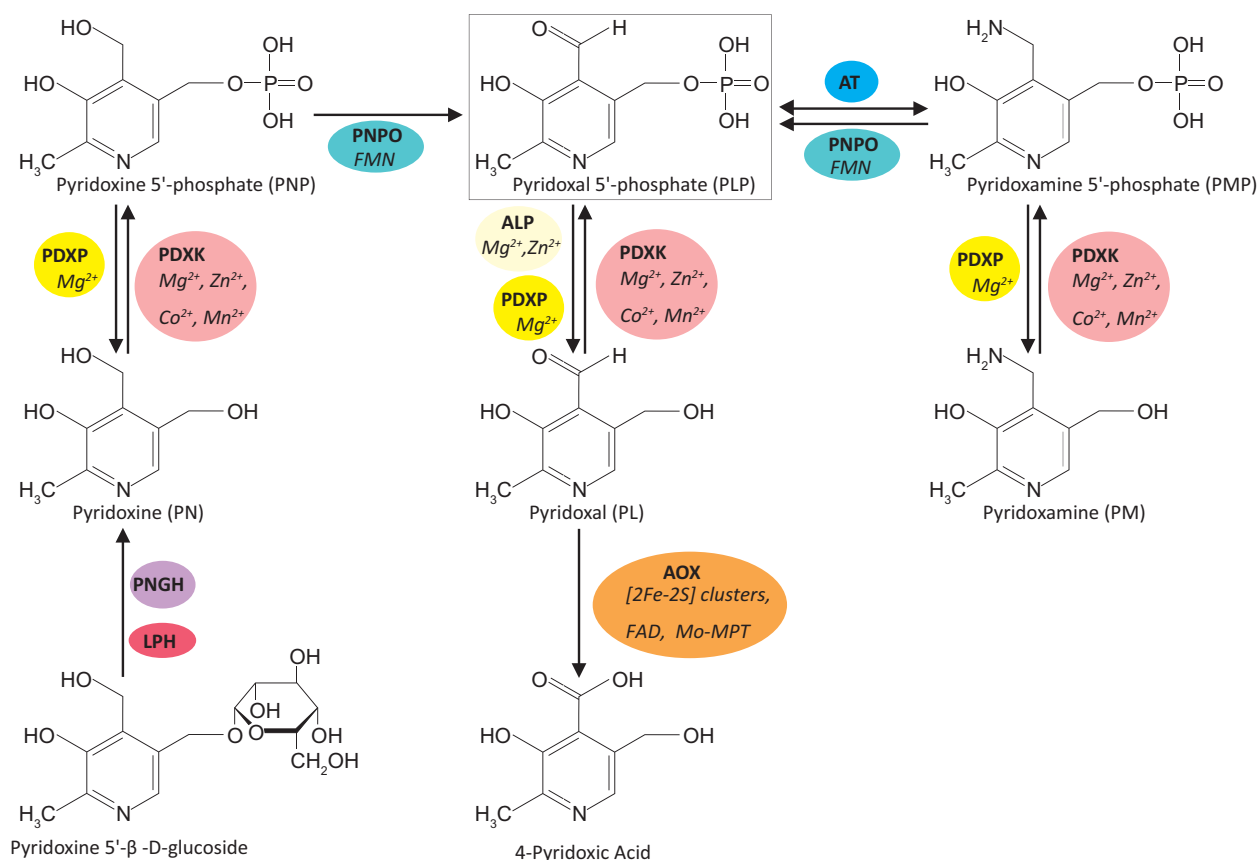
Figure 1 – Mutual conversion of three B 6 vitamers
